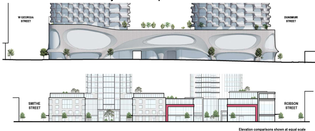
Figure 2 - Proposed Richards Street frontage compared with typical nearby Downtown podium conditions
