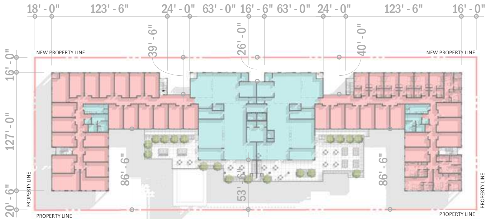
TYPICAL FLOOR PLAN TO SHOW DEEP INDENTATION ALONG GRANVILLE STREET TO BREAK UP THE MASSING. REFER TO SHEET A3.4 FOR THE SAME INDENTATION SHOWN ON LANE.
