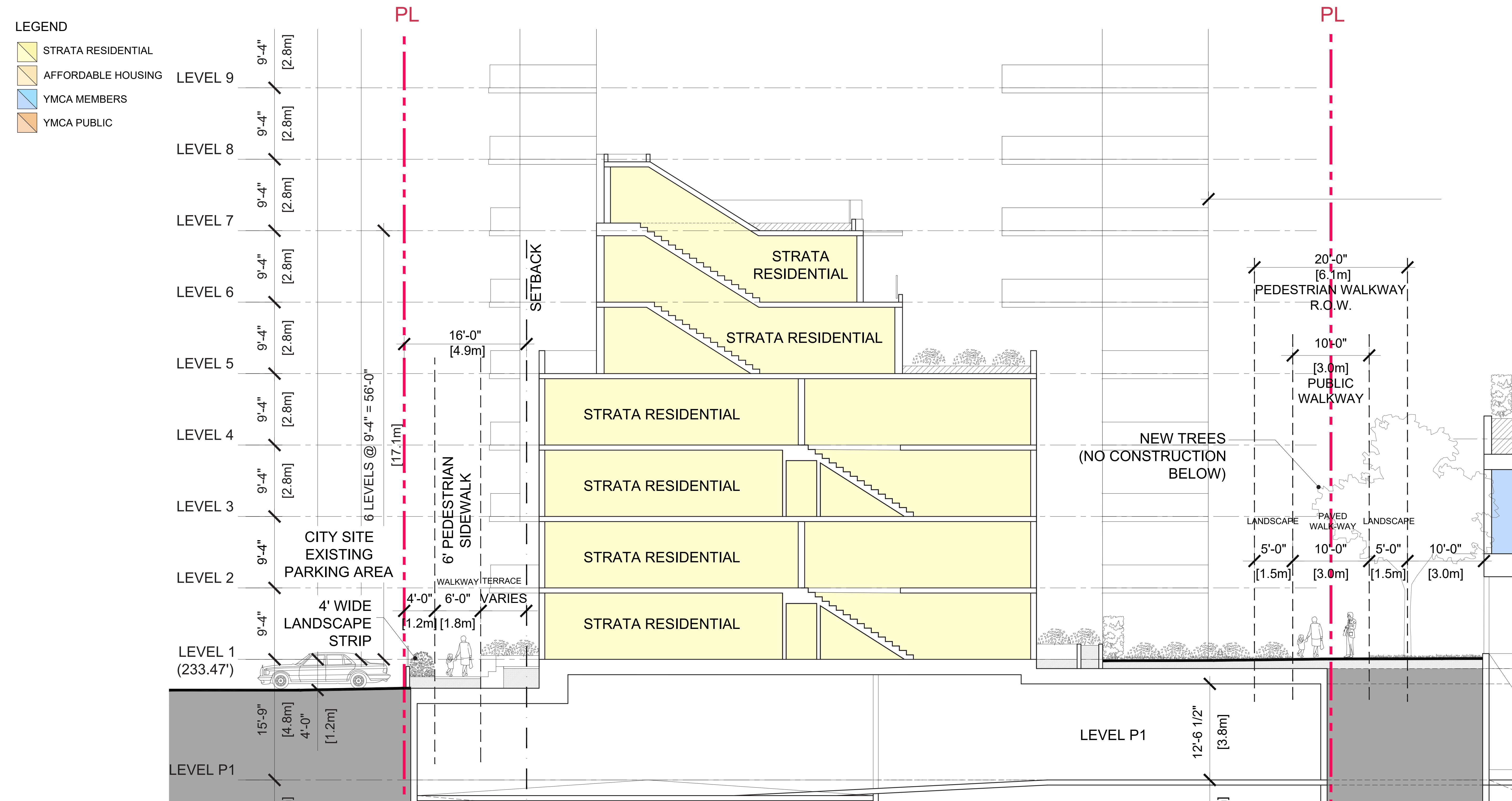
Detail Section at South Property Line & Mid-site Pedestrian Walkway
