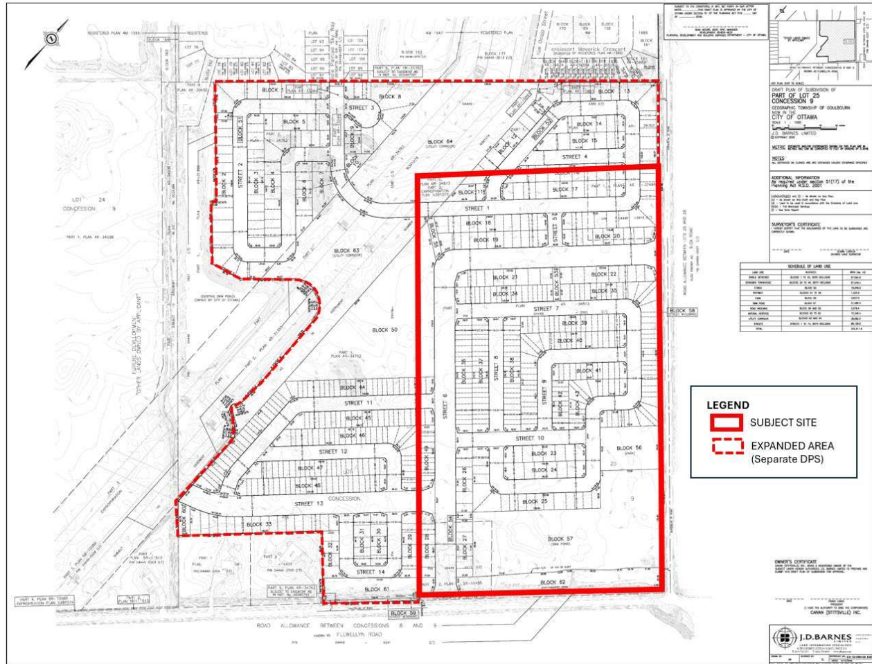
Figure 9 – Draft Plan
