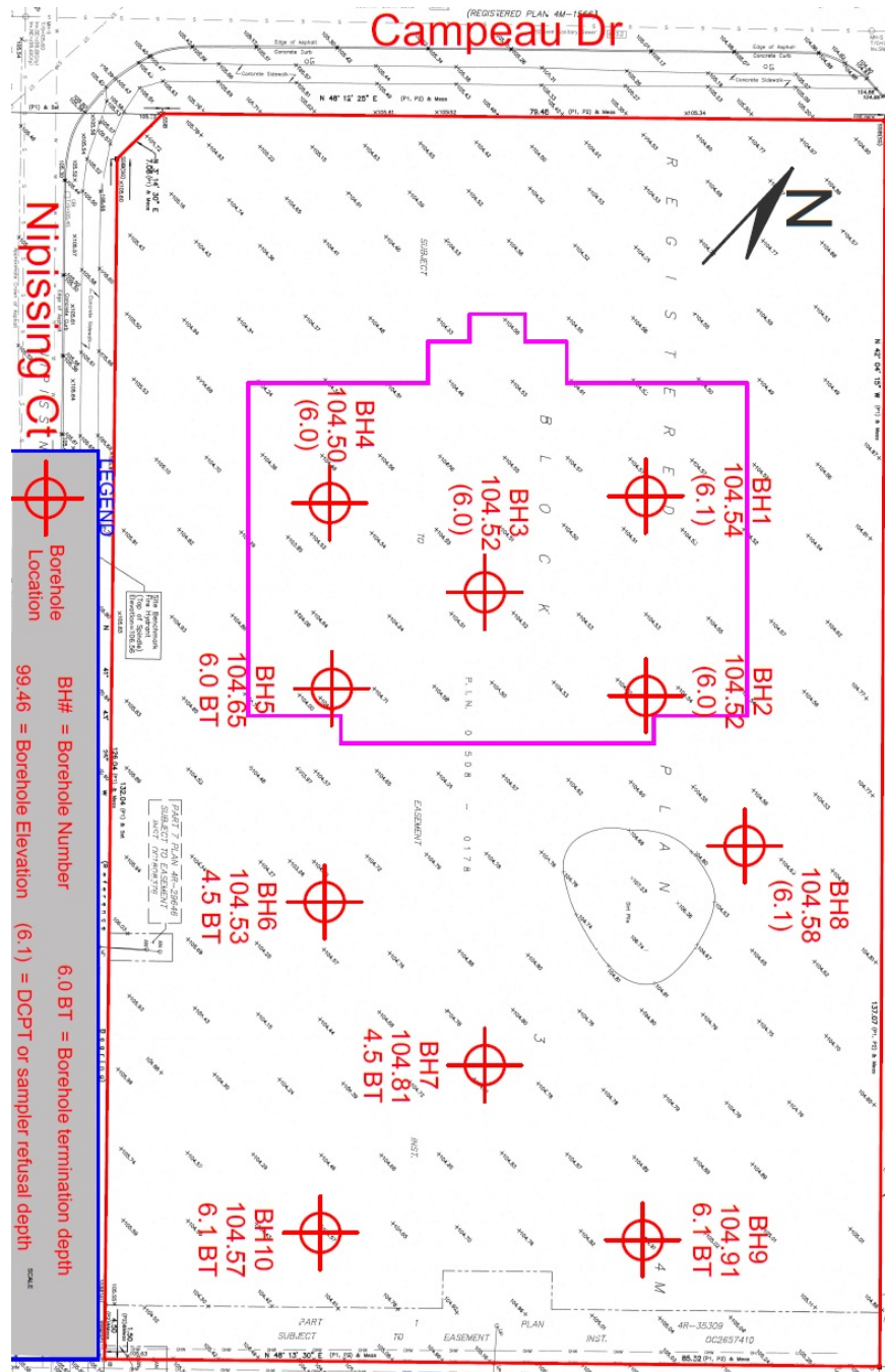
Figure 1: Test hole Locations Plan
