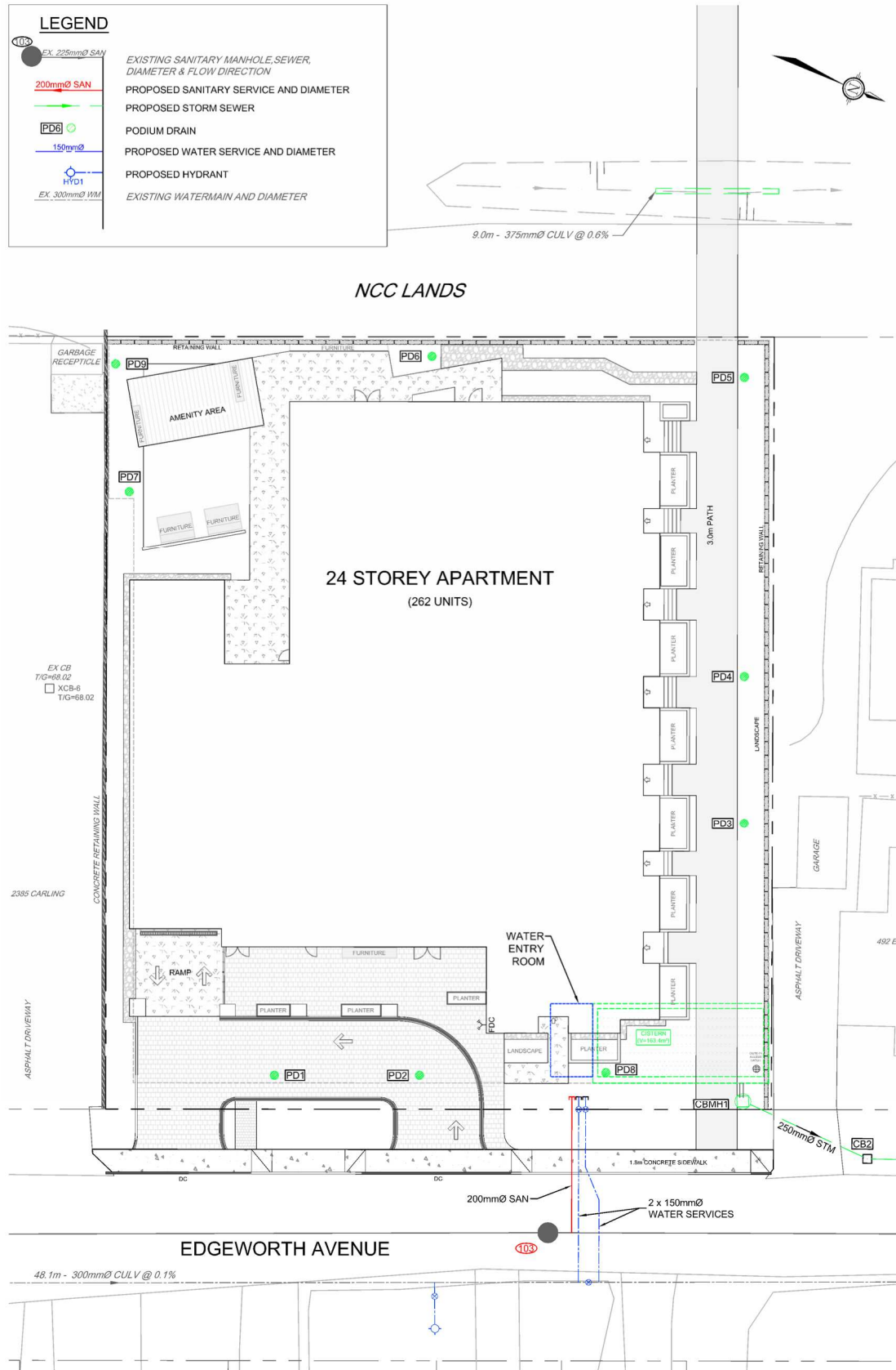
Figure 3-1: Proposed Servicing Schematic
