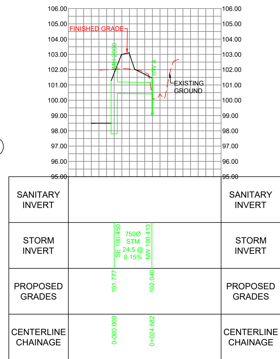
4000 EAST POND OUTLET
