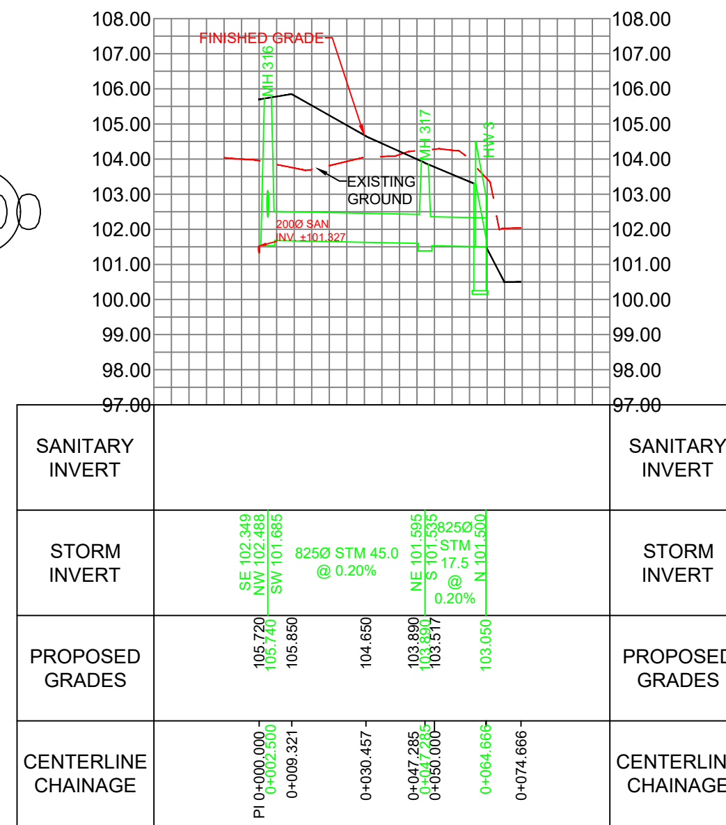
3000 DAVIDSON POND INLET
