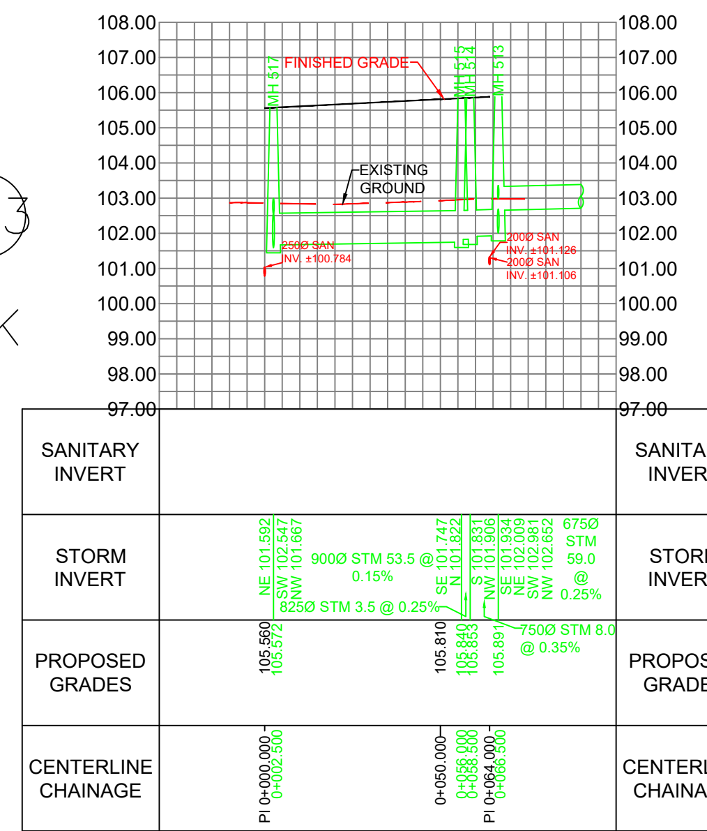
503 SERVICING BLOCK
