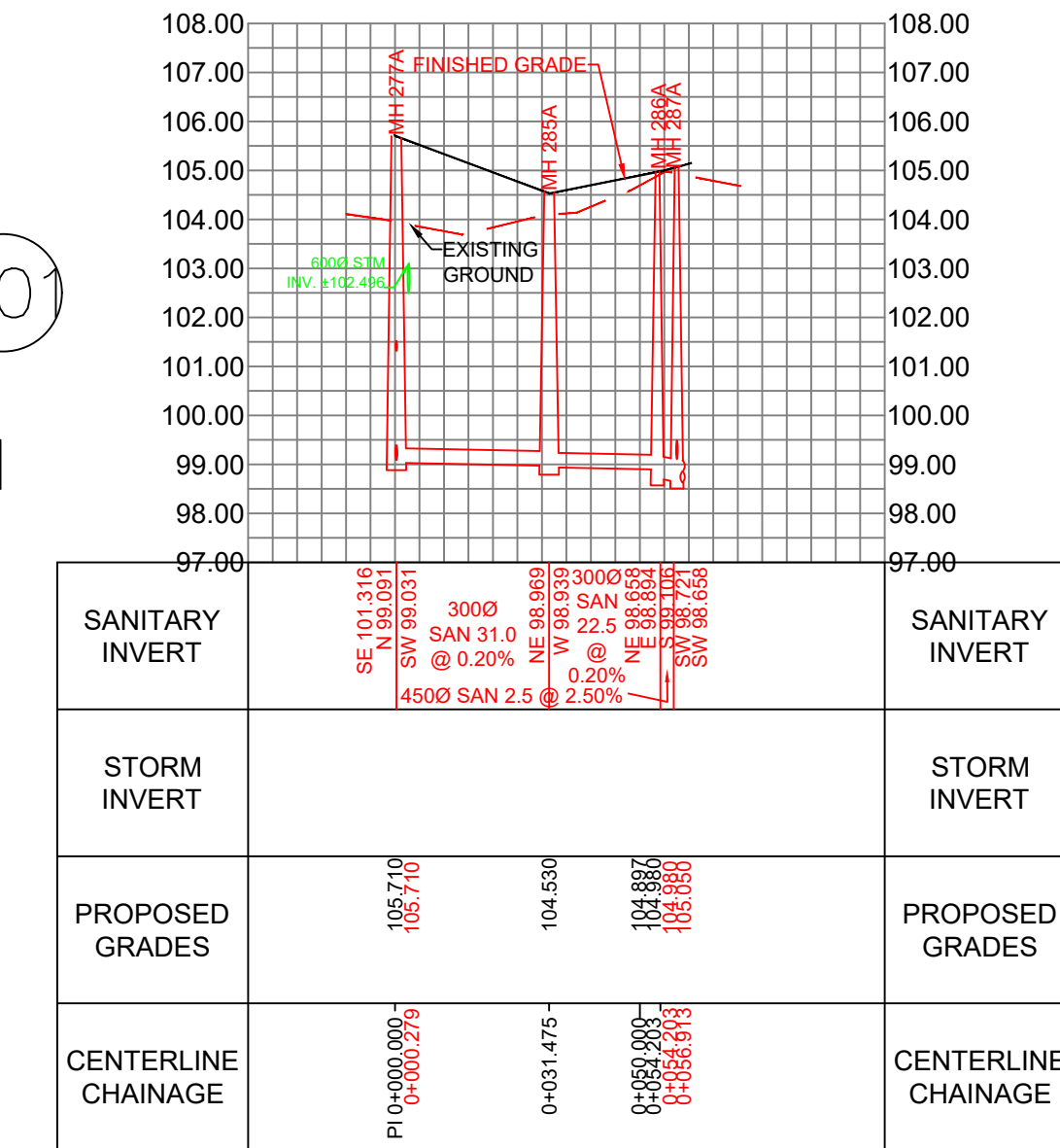
201 PUMP STATION INLET 2
