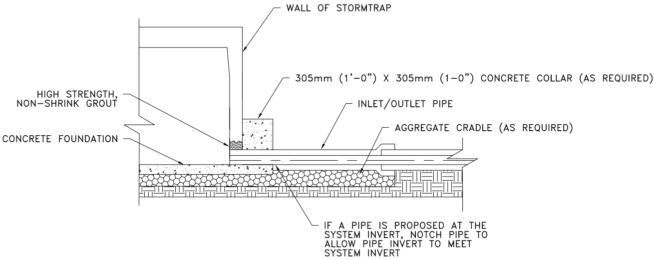
NOTCHED PIPE CONNECTION DETAIL WHEN PIPE INVERT IS AT INVERT OF STORMTRAP SYSTEM
