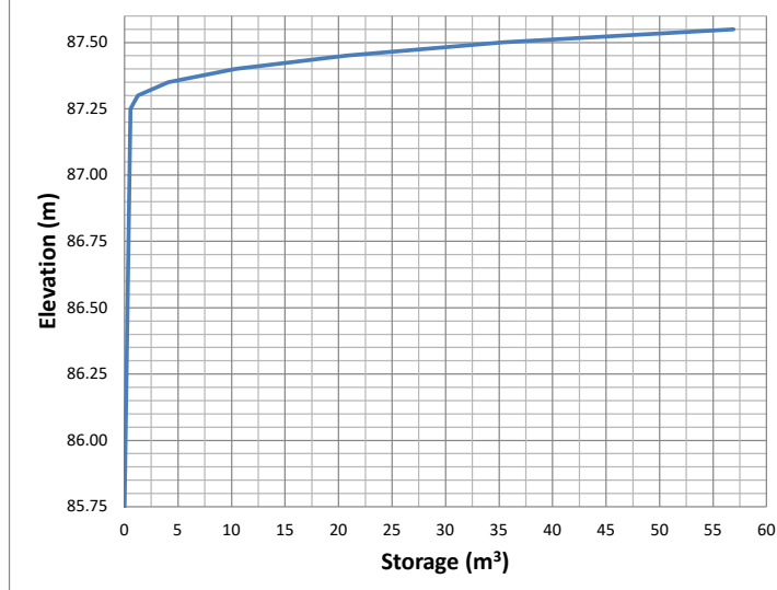
Stage Storage Curve Area A-03 (CB 01)
