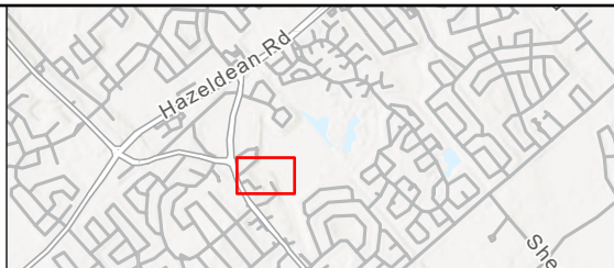
Figure 2. Boundary trees
