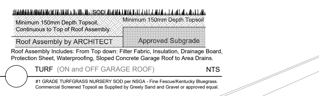
TURF (ON AND OFF GARAGE ROOF) Section
