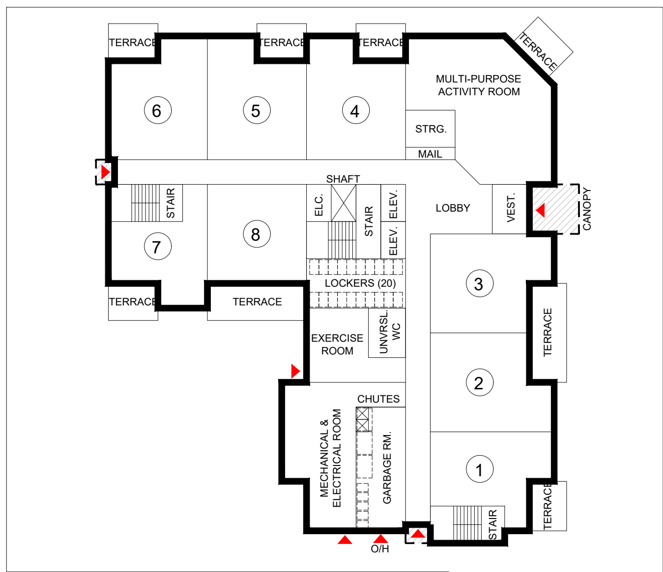
5 Phase 3 - Ground Floor Plan A2.2 1:300
