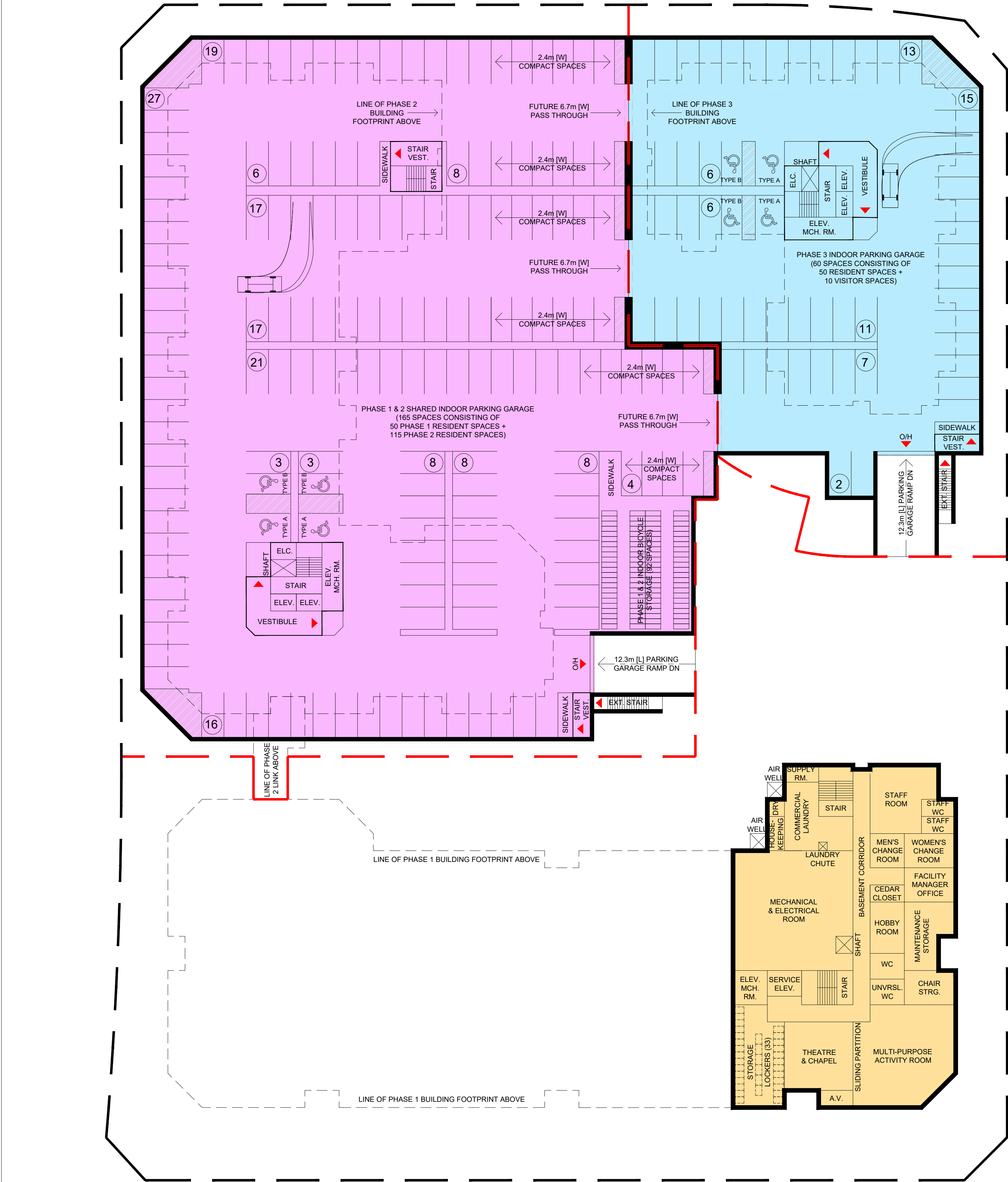
1 Phase 1 - Basement Floor Plan / Phase 2 & 3 Underground Parking Garage Plan A2.0 1:300
