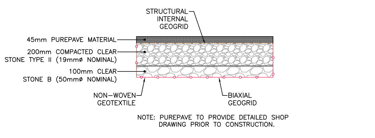
PUREPAVE DETAIL FOR SIDEWALK AREAS N.T.S.
