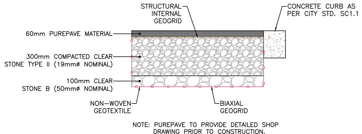
PUREPAVE DETAIL FOR PAVEMENT AREAS N.T.S.
