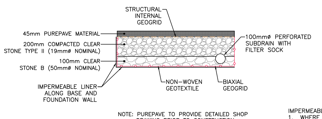
PUREPAVE DETAIL FOR SIDEWALK AREAS WITH PERFORATED SUBDRAIN/IMPERMEABLE LINER N.T.S.
