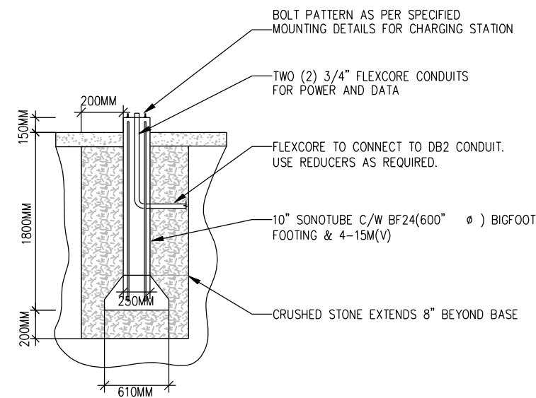
3 EV CHARGER BASE DETAIL SCALE:1:150
