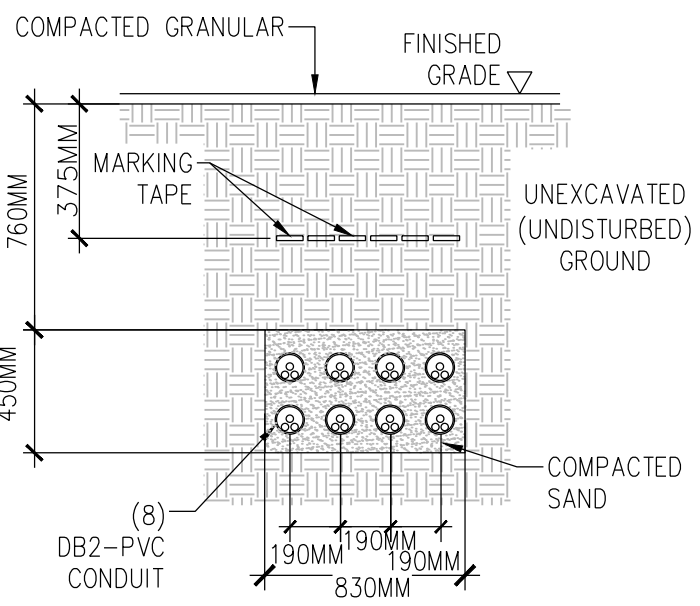
5 COMPACT SAND DUCT BANK DETAIL SCALE:1:100
