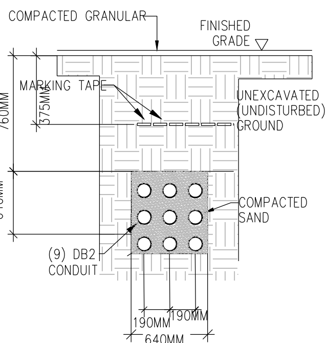
4 DUCT BANK DETAIL SCALE:1:100
