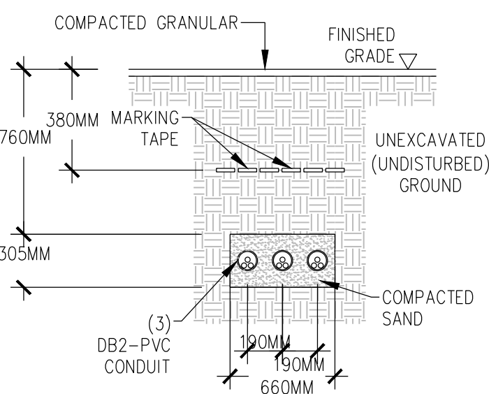
7 COMPACT SAND DUCT BANK DETAIL SCALE:1:100
