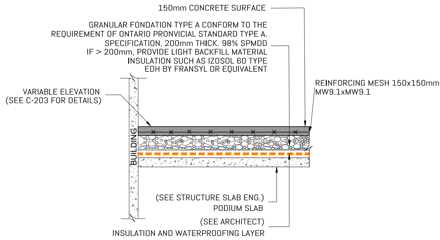
SIDEWALK SECTION ON PODIUM SLAB
