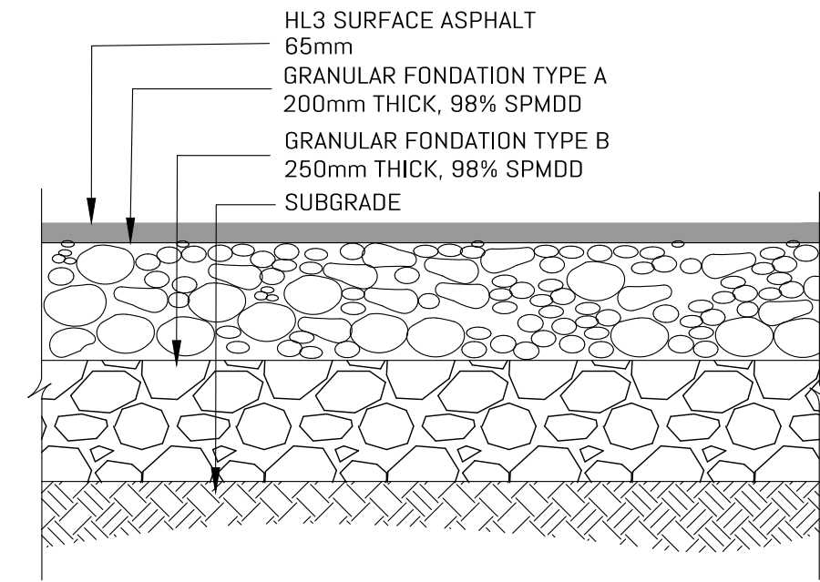
PARKING AND ACCESS FOUNDATION ASPHALT SURFACE
