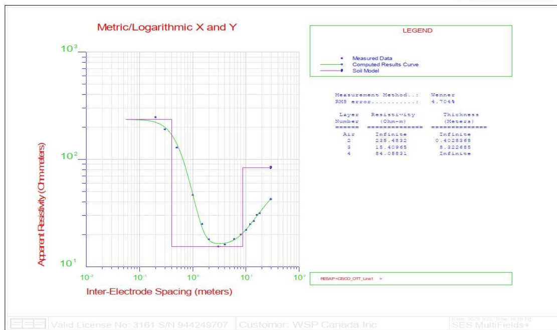
Figure 4: Soil Electrical Resistivity Model Based On Measured Data of VES Line 1
