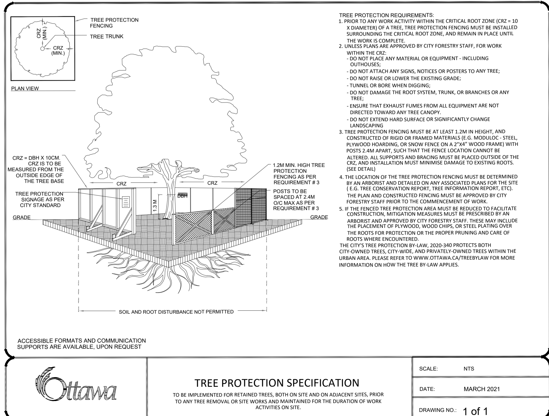
1 TREE PROTECTION FENCING T-201
