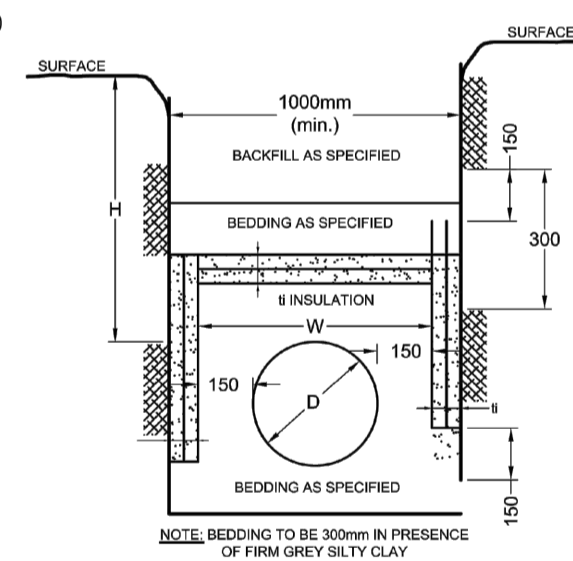
INSULATION DETAIL FOR SHALLOW SEWERS & WATERMAIN
