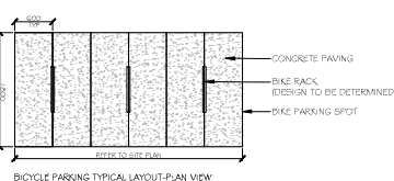
BICYCLE PARKING TYPICAL LAYOUT-PLAN VIEW
