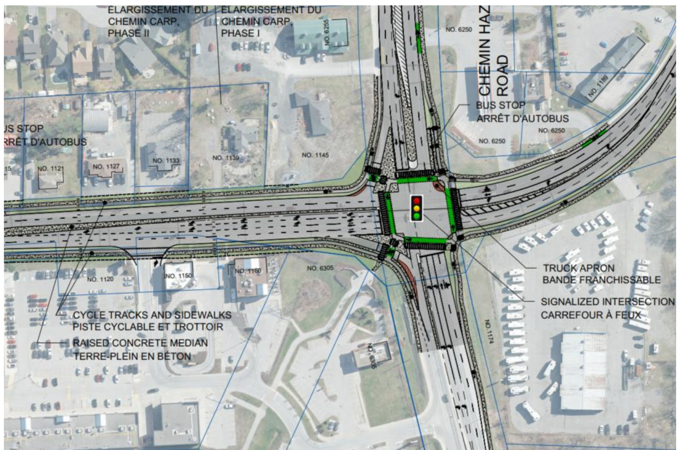
Figure 2: Carp Road Widening at Hazeldean Road
