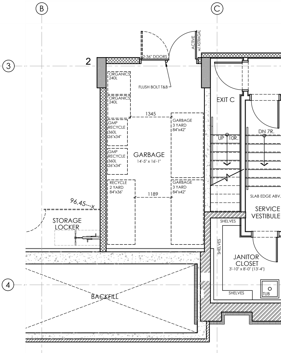
PARTIAL P1 LEVEL PLAN - GARBAGE ROOM LAYOUT SCALE = 1:75
