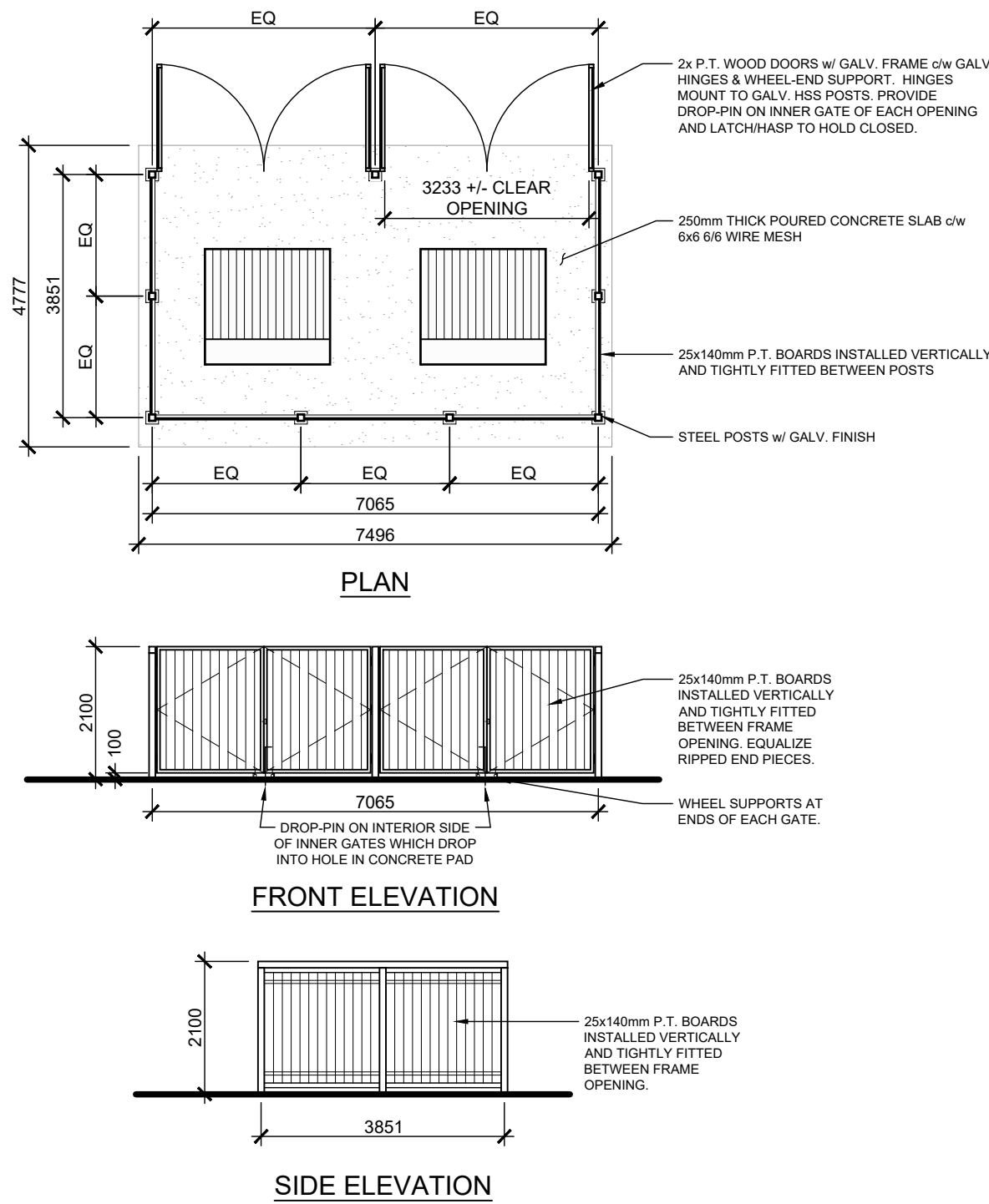
07 SHOP DRAWING DETAIL - WASTE ENCLOSURE SP-A04 SCALE: 1:100
