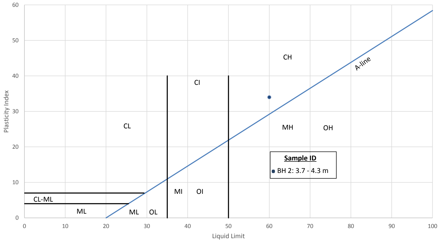
Plasticity Chart
