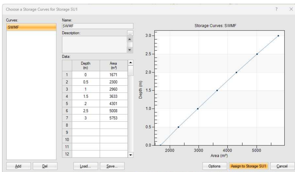
Figure 16: PCSWMM Storage curve
