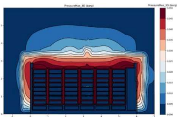
Figure 4-8: Top front center ignition pressure map (outside).
