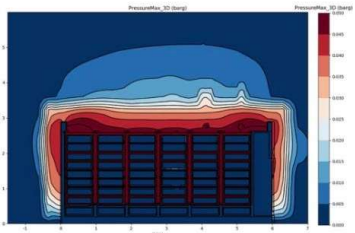
Figure 4-9: Top front corner ignition pressure map (outside).
