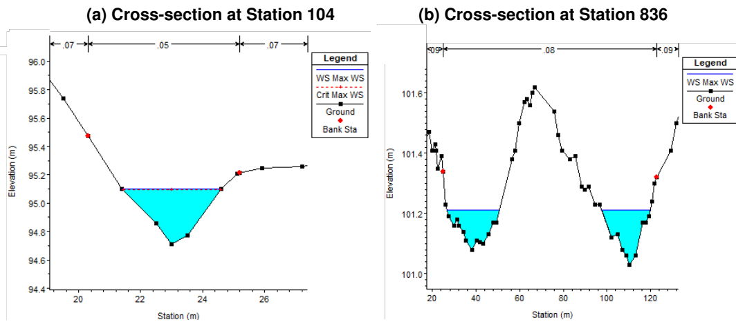
Figure 4-2: Cross-sections with Critical Flow for 100-year Storm Event
