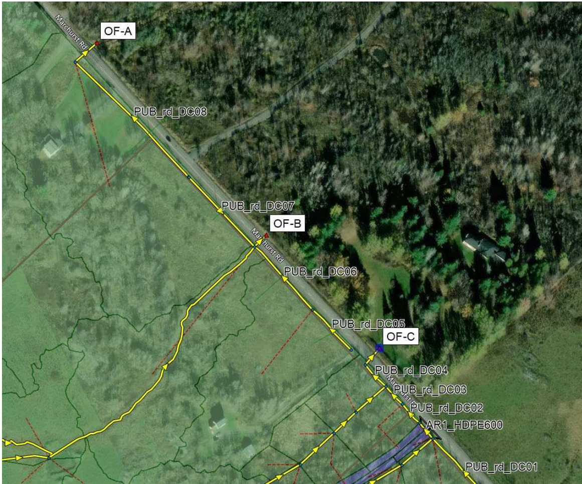
Figure 4: Layout with section ID public road ditch
