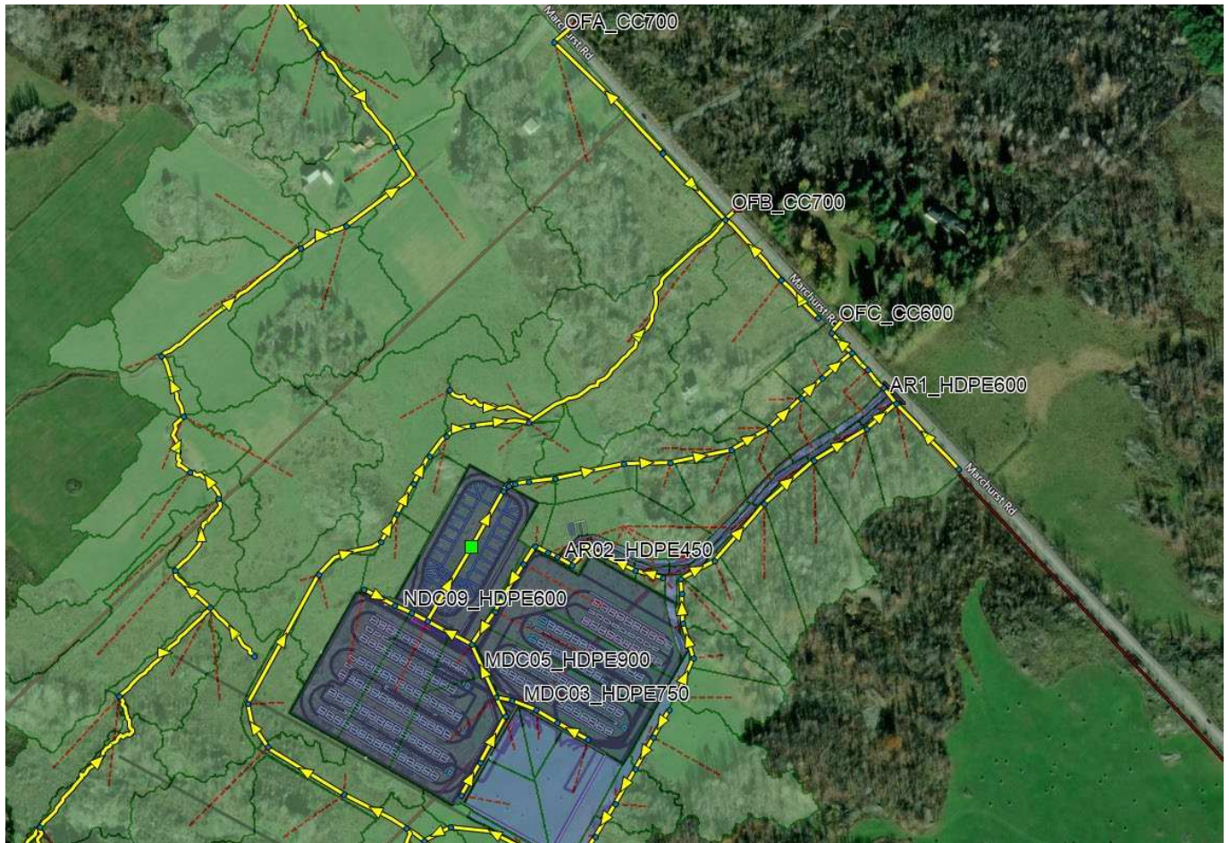
Figure 3: Layout with conduit ID of culverts (proposed and existing culverts)
