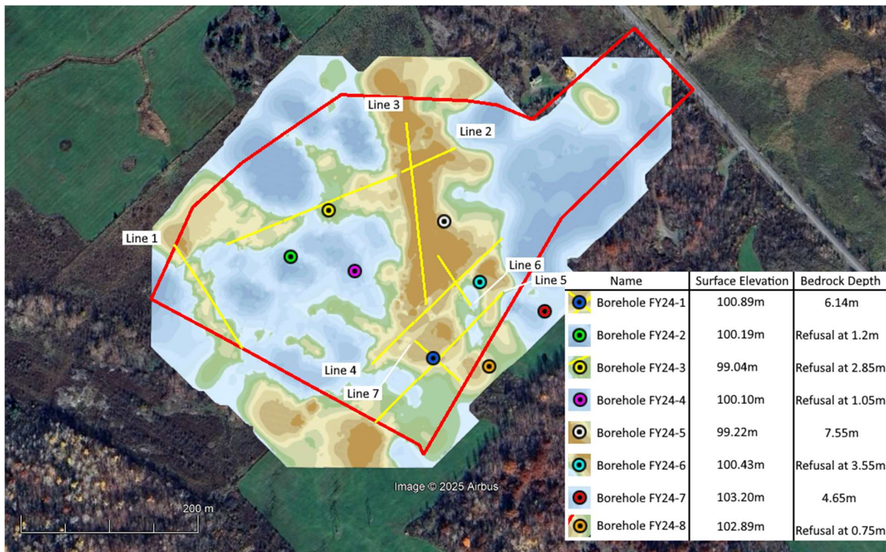
Figure 8: EM-31 In-Phase Magnetic Susceptibility Map with Seismic Line and Borehole Overlay
