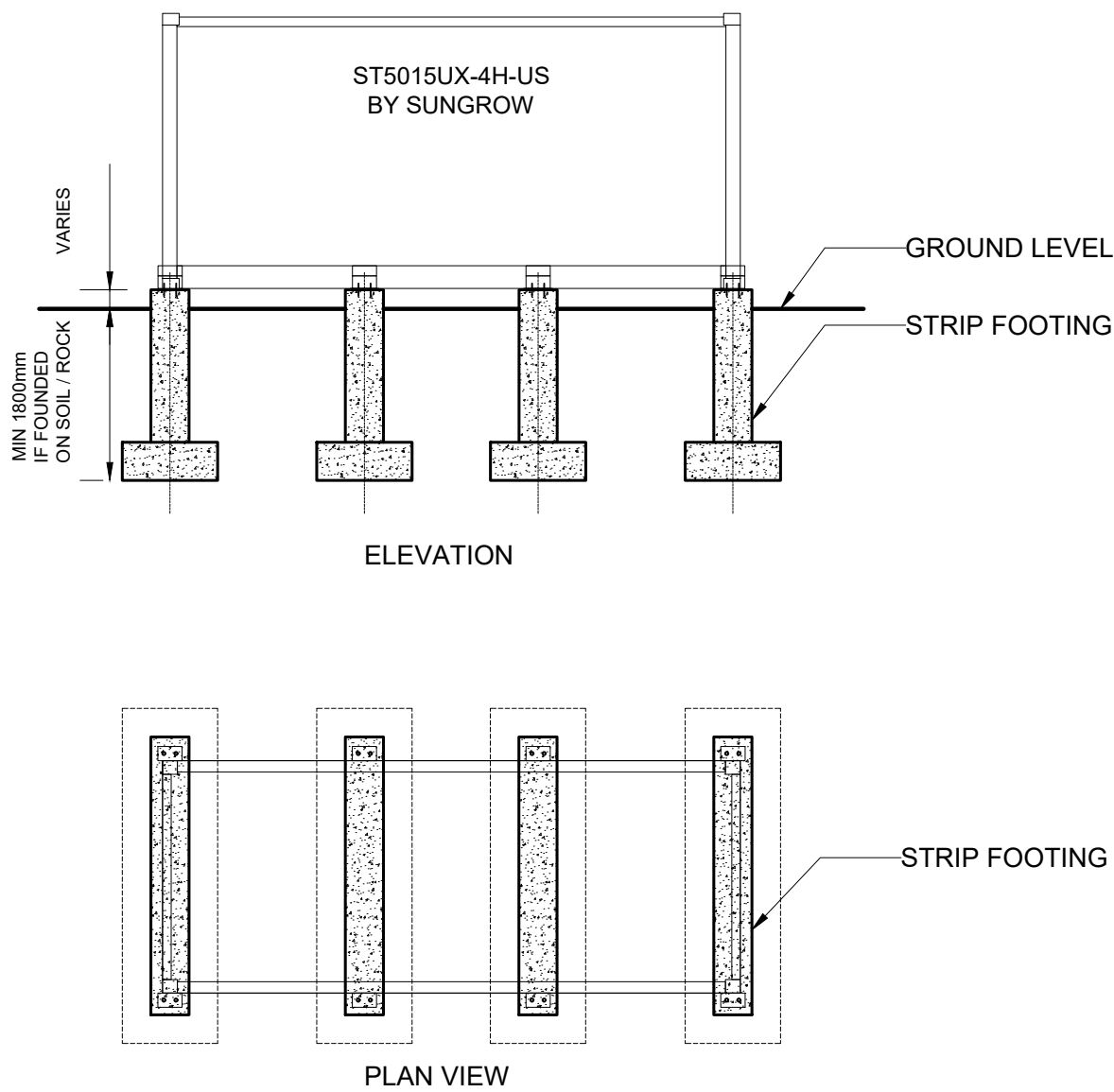
TYPE 3: CONCRETE STRIP FOOTING ACROSS THE LENGTH
