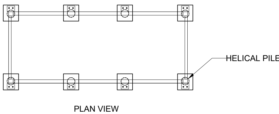
TYPE 2: HELICAL PILE
