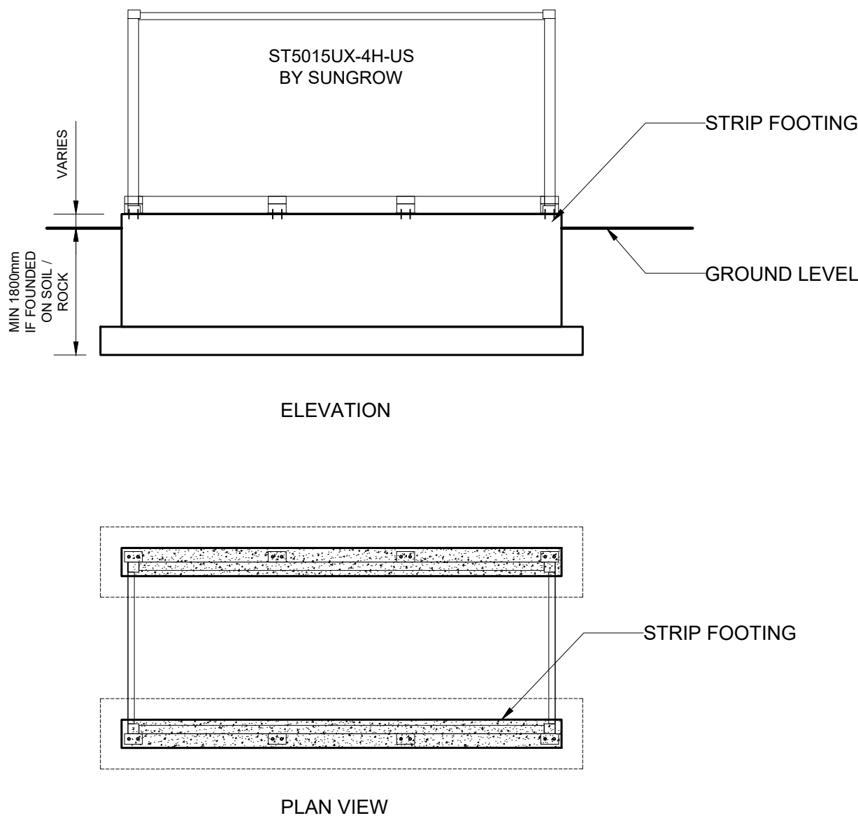
TYPE 4: CONCRETE STRIP FOOTING ALONG THE LENGTH
