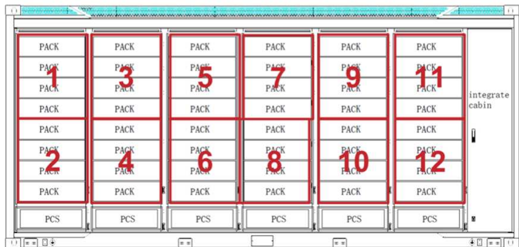
Figure 2-1: Battery Energy Storage System Geometry
