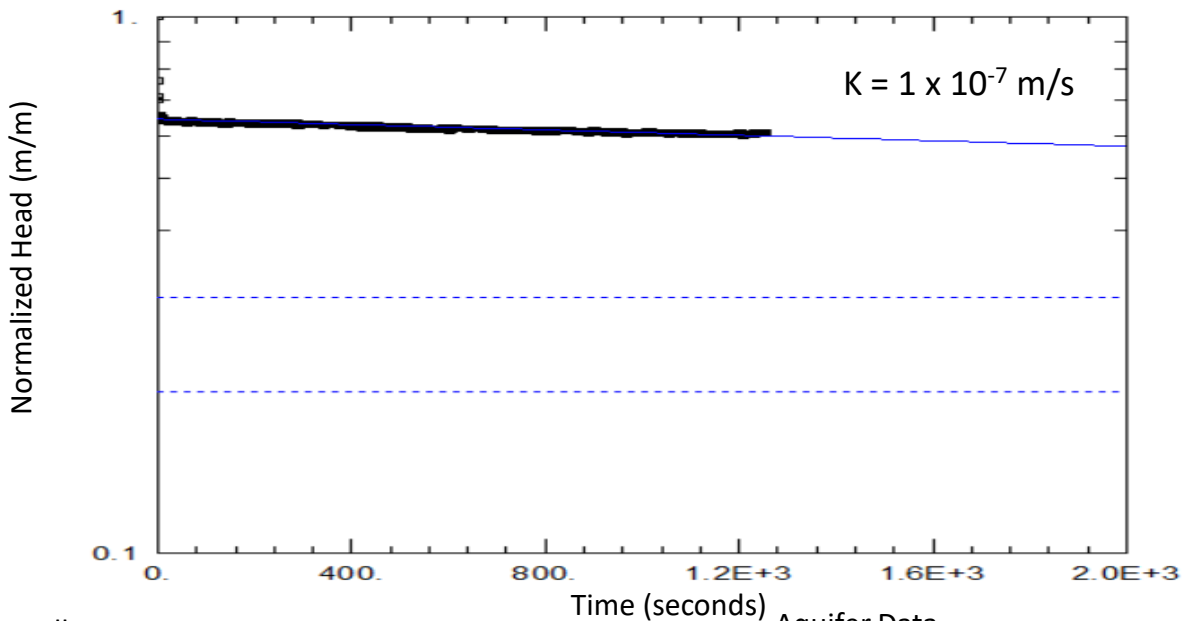
Borehole 23-03A FH: Bouwer-Rice Analysis
