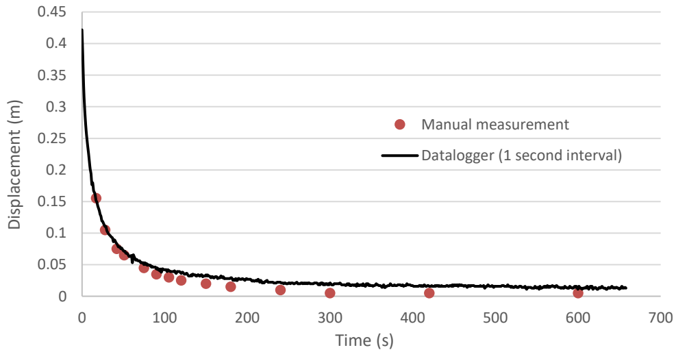
Borehole 23-03B FH: Bouwer-Rice Analysis
