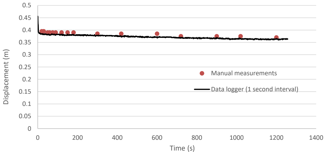
Borehole 23-03A FH: Bouwer-Rice Analysis
