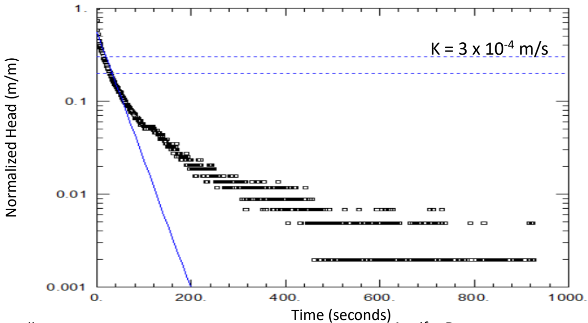
Borehole 23-03B FH: Bouwer-Rice Analysis
