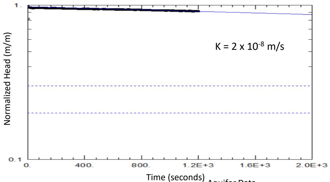
Borehole 23-02 FH: Bouwer-Rice Analysis
