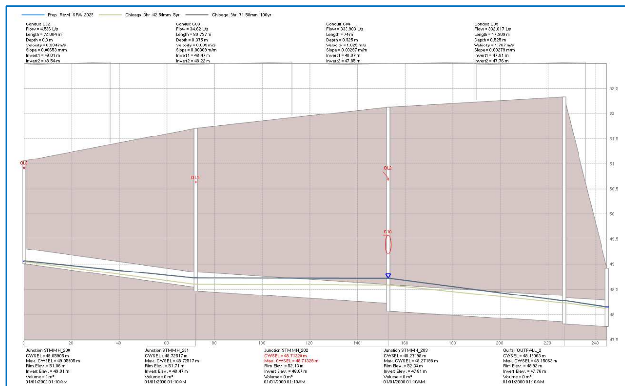
Figure 7-1: Hydraulic Grade Lines of 5-yr and 100-yr Storms of Jeanne-d’Arc Storm Sewers
