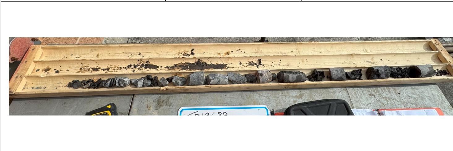
Borehole 25-08 Depth: 17.8 m – 19.4 m Bedrock, Run1, RQD 0%
