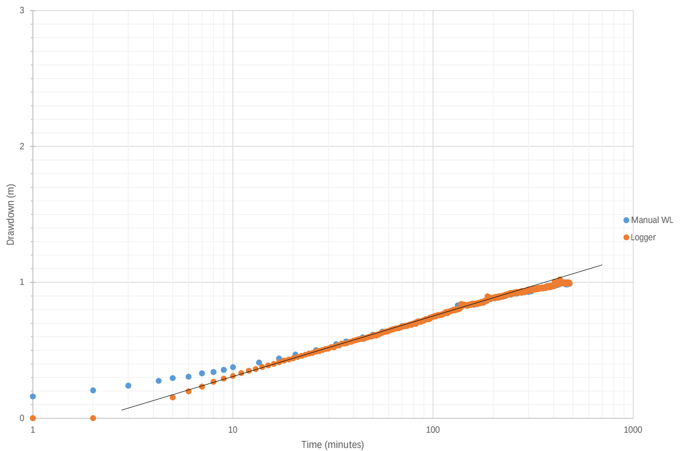
Drawdown vs Log Time Pumping Test (Drawdown)
