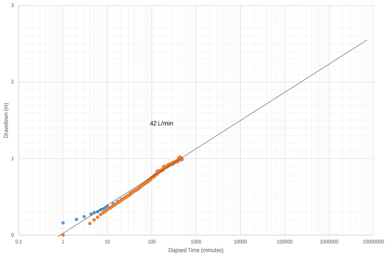
Drawdown vs Log Time Pumping Test (Long-Term)
