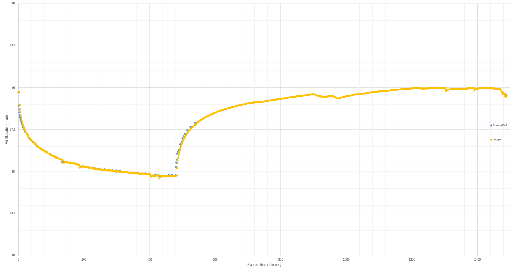
Water Level Elevation vs Time Pumping Test (Drawdown and Recovery)
