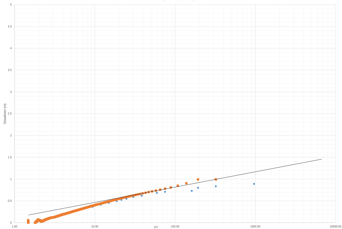
Drawdown vs Log Time Pumping Test (Recovery)
