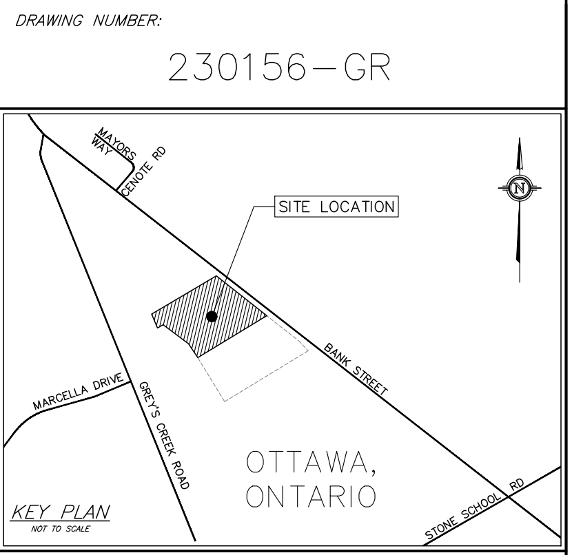
DRAWING: GRADING AND DRAINAGE PLAN
