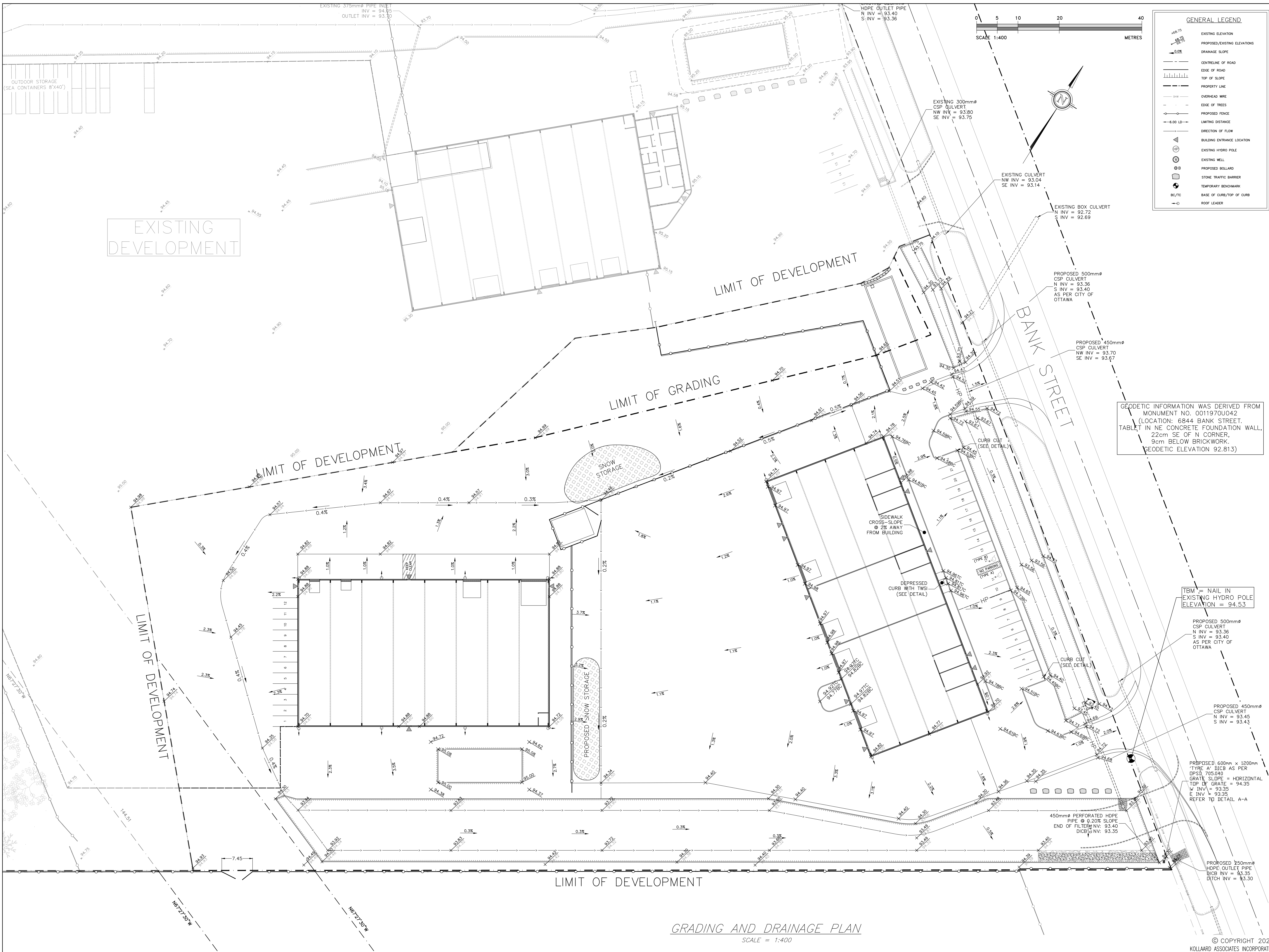
DRAWING: GRADING AND DRAINAGE PLAN
