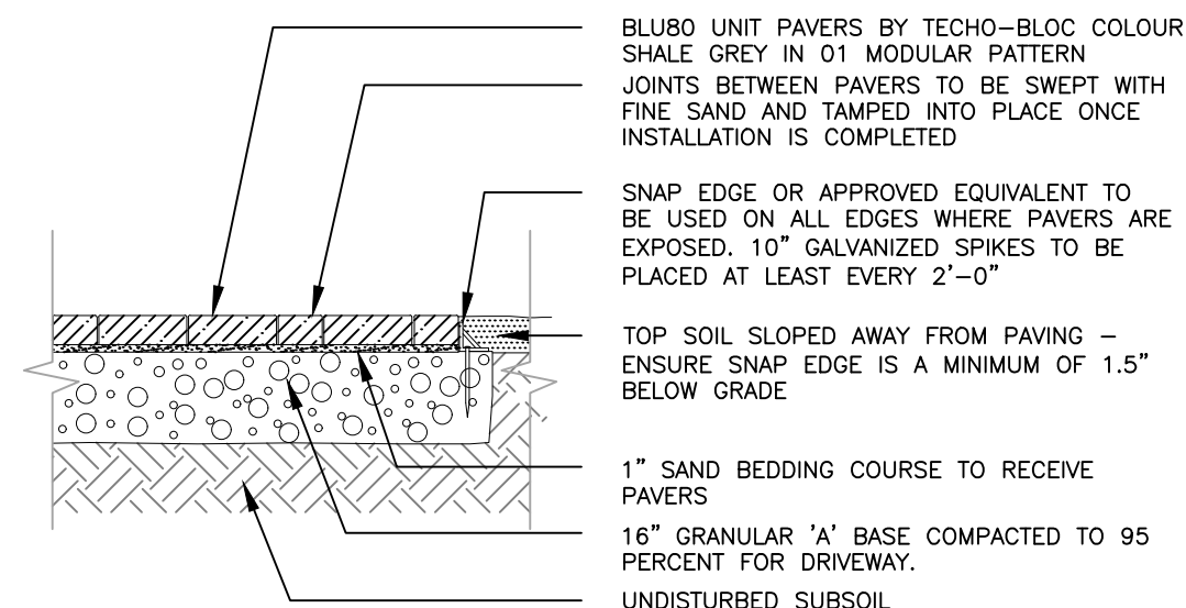
5 L1 UNIT PAVING - DRIVEWAY n.t.s.
