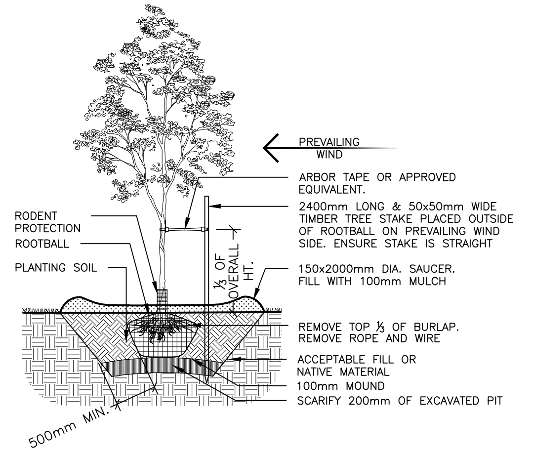
1 L1 DECIDUOUS TREE PLANTING n.t.s.
