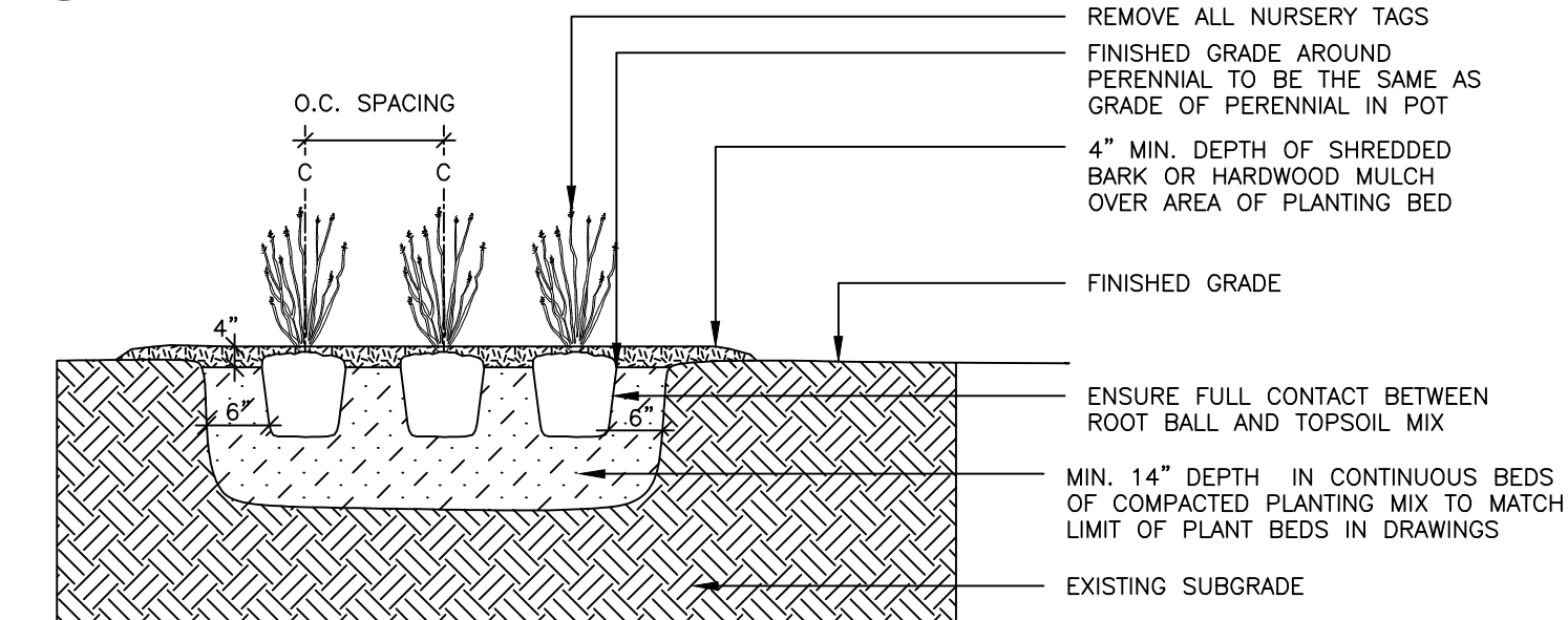
2 L1 SHRUB PLANTING n.t.s.
