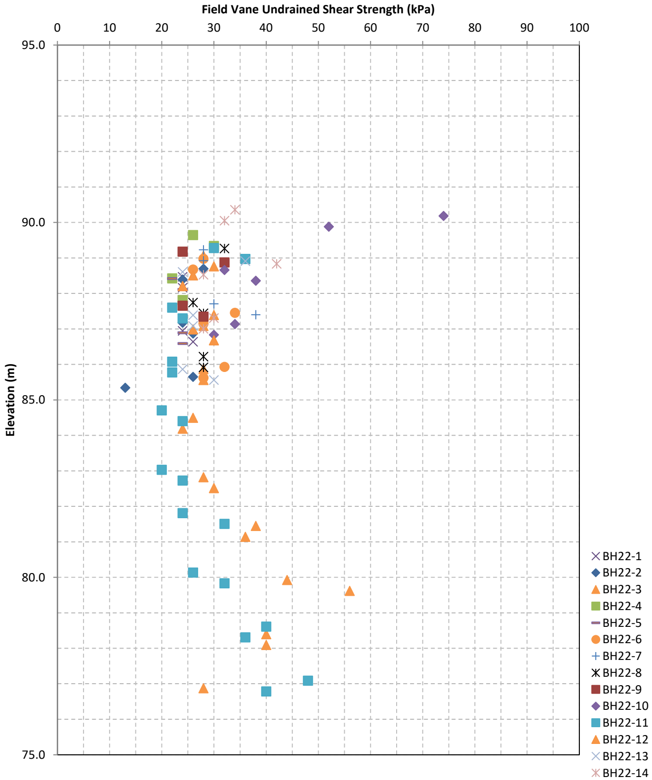
FIGURE 3 PROPOSED 3850 CAMBRIAN ROAD DEVELOPMENT 2022 GEOTECHNICAL INVESTIGATION FIELD VANE DATA VERSUS ELEVATION
