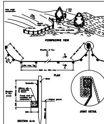
LIGHT-DUTY SILT FENCE BARRIER
