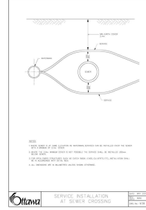
SERVICE INSTALLATION AT SEWER CROSSING
