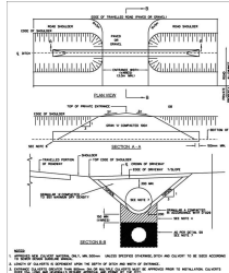
PRIVATE ENTRANCE DETAIL - TYPICAL
