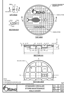
STANDARD CIRCULAR STORM MAINTENANCE HOLE COVER
