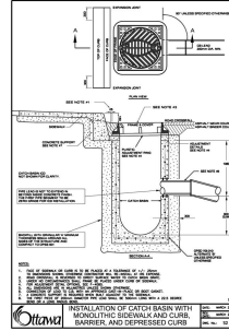
INSTALLATION OF CATCH BASIN WITH MODULAR SIDEBOARD AND CURB BARRIER AND DEPRESSION CURB
