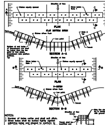
STRAW BALE FLOW CHECK DAM
