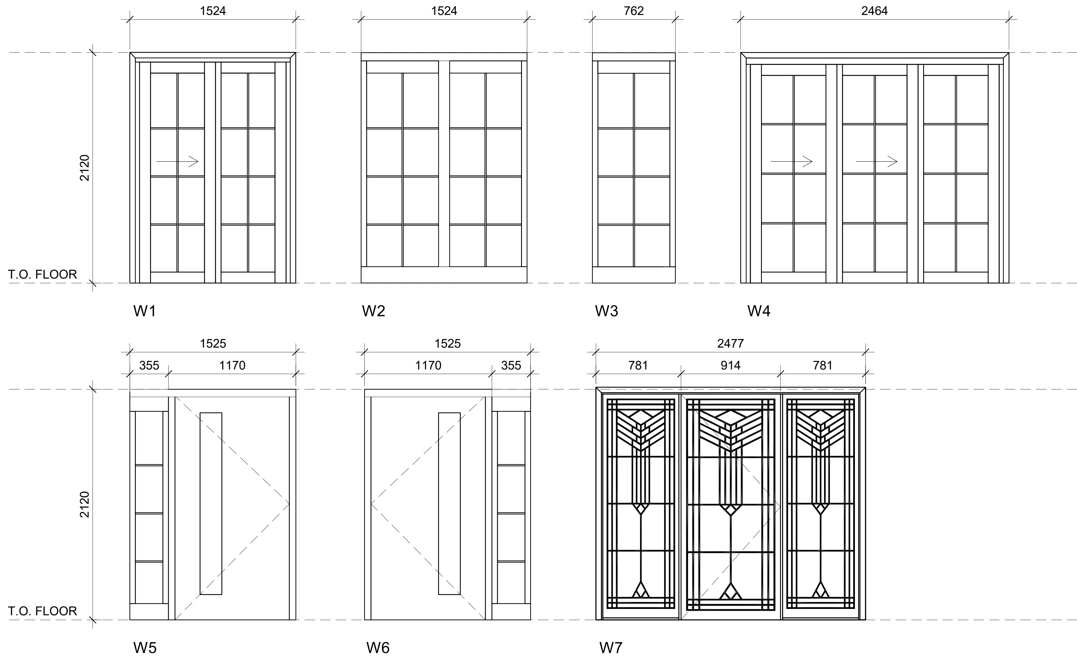
Window schedule 1 : 20
