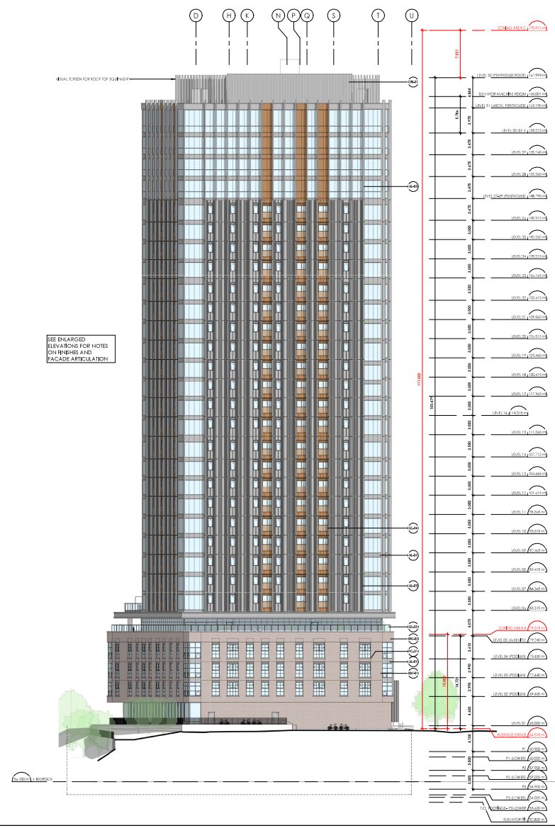
2 BUILDING ELEVATION - NORTH
