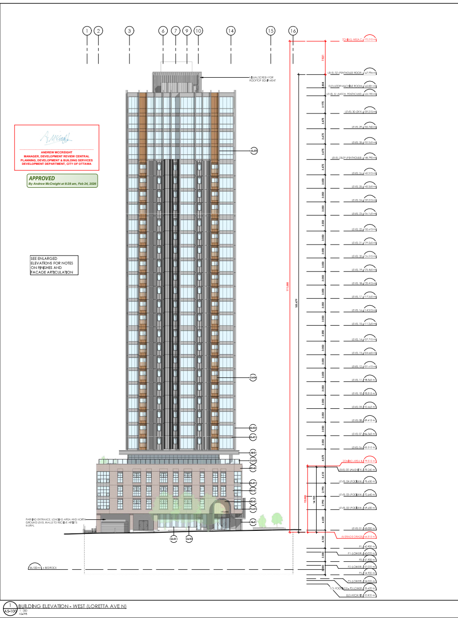
1 BUILDING ELEVATION - WEST (LORETTA AVENUE) 1/80
