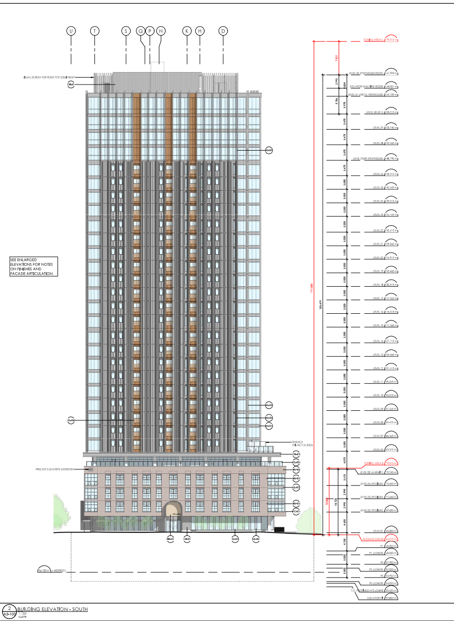
2 BUILDING ELEVATION - SOUTH 1/80
