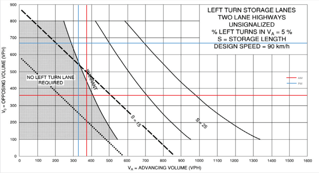
Blais at Hawthorne Future Total 2036 - Northbound Left
