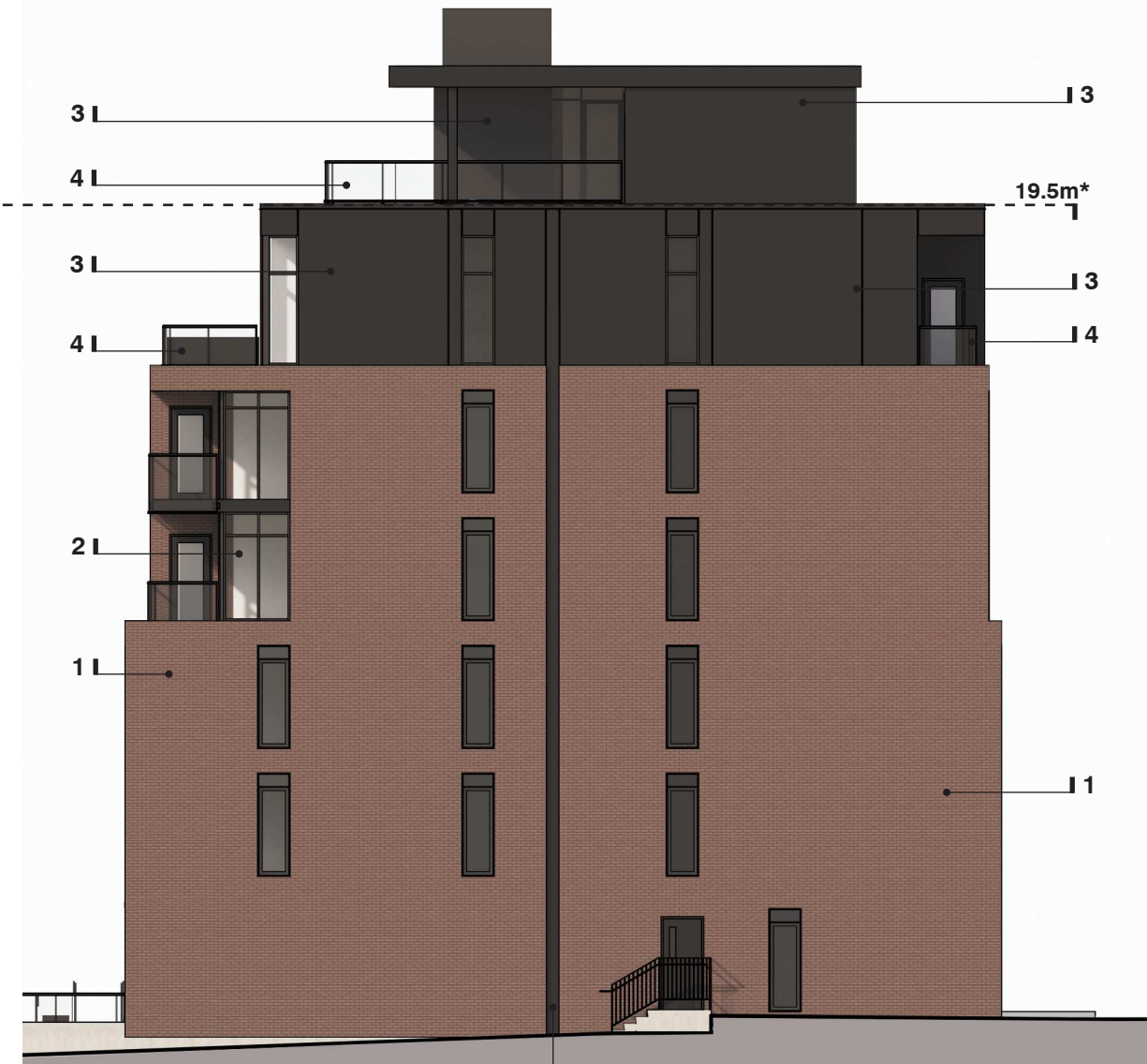
South Elevation
