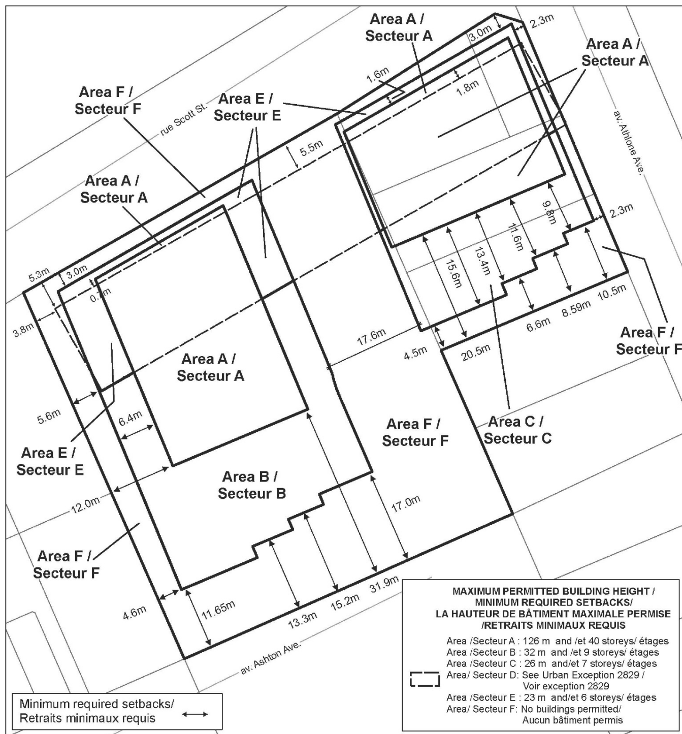
Figure 19: Schedule 465, identifying the existing built form provisions and setbacks of the subject property.
