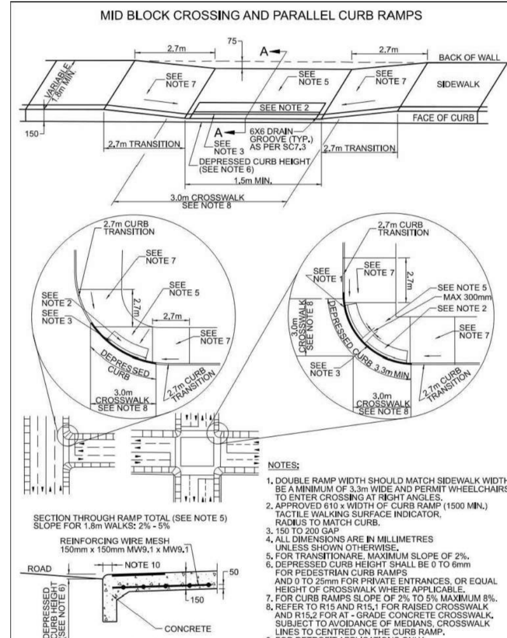
SECTION A-A SECTION B-B DATE: MAY 2001 REV: MARCH 2023 DWG. No.: SC6
