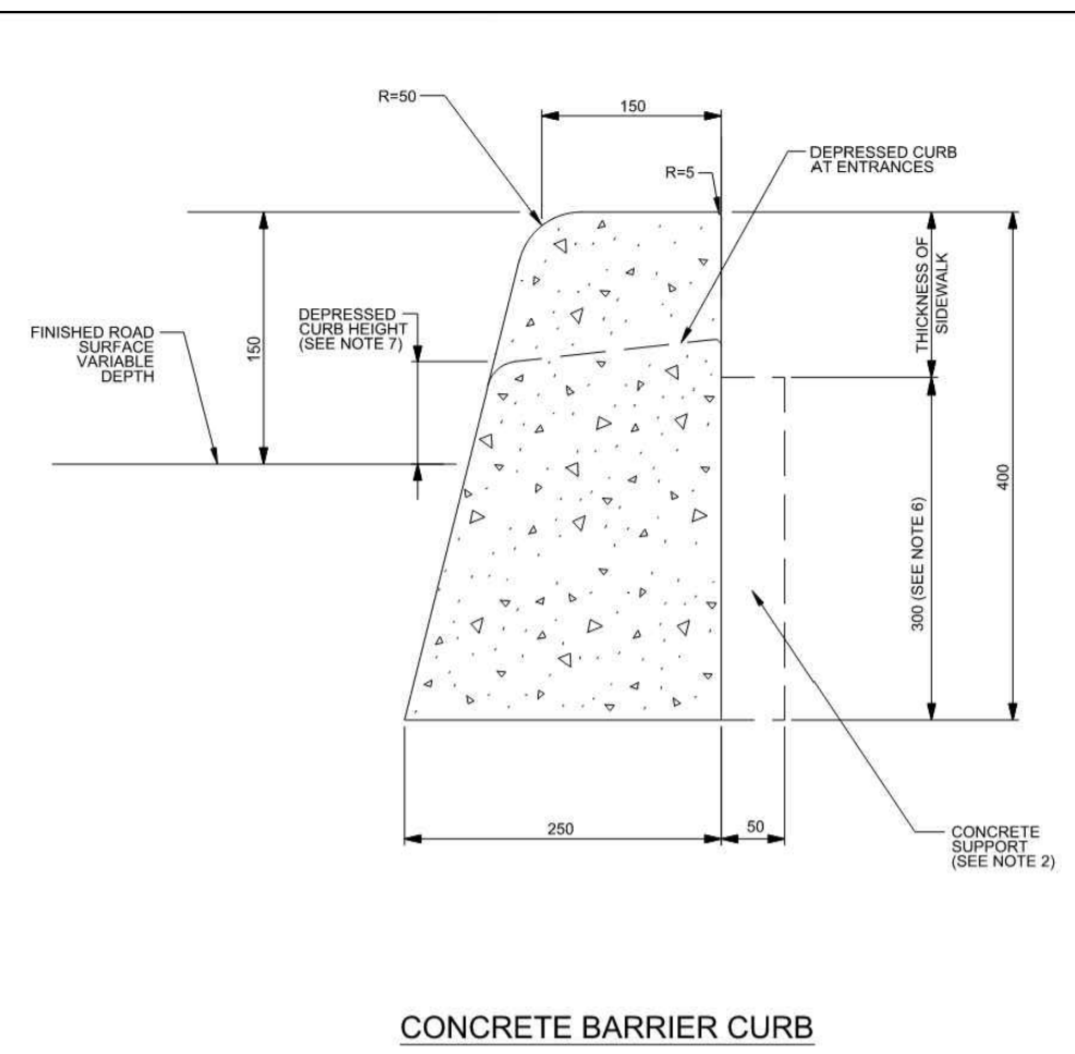
CONCRETE BARRIER CURB
