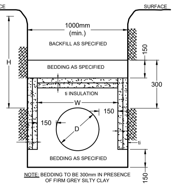
INSULATION DETAIL FOR SHALLOW SEWERS & WATERMAIN N.T.S.
