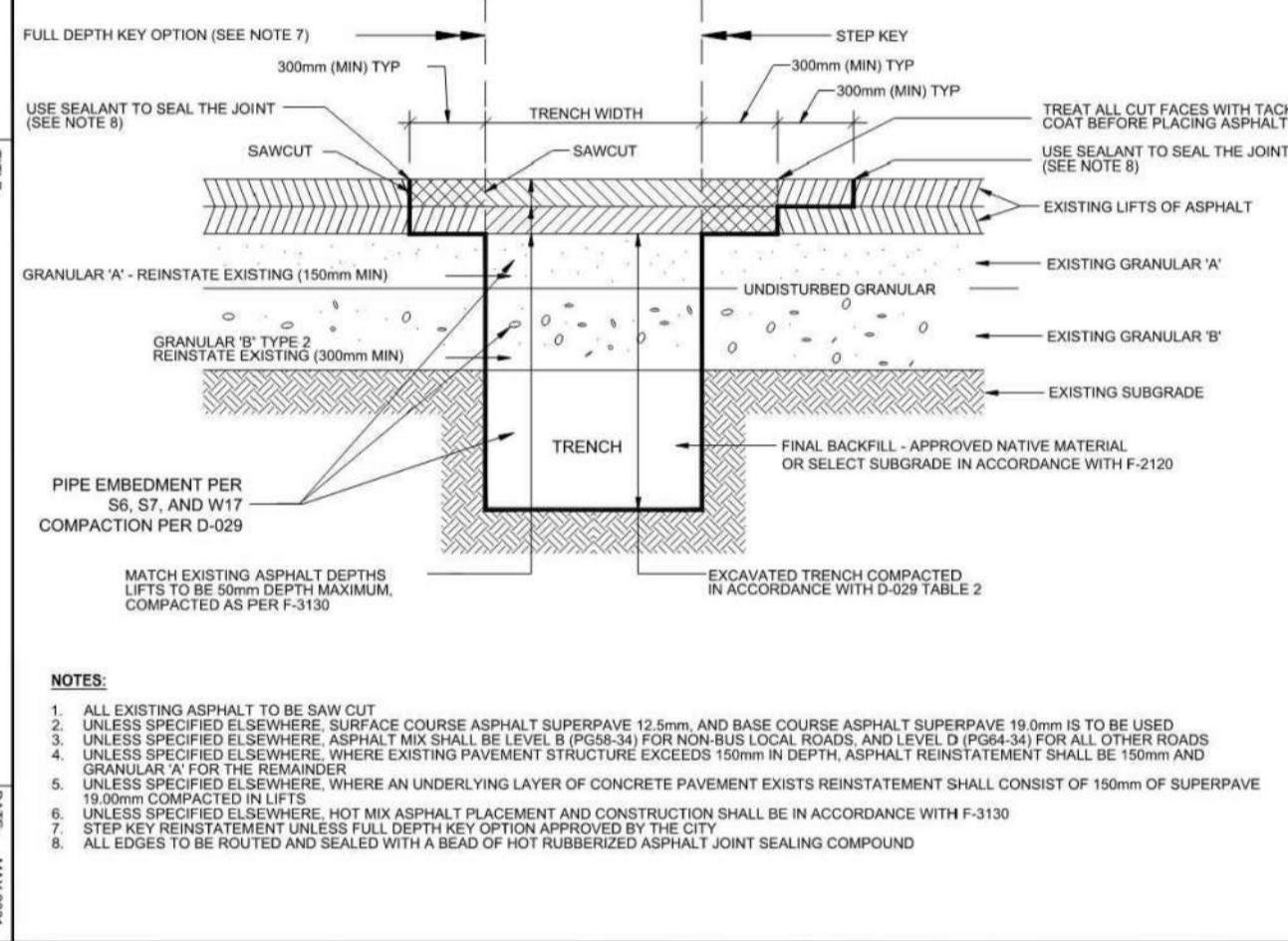
SECTION A-A SECTION B-B DATE: MAY 2020 REV: MARCH 2020 DWG. No.: R10
