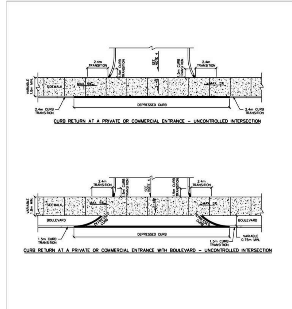
SECTION A-A SECTION B-B DATE: MARCH 2007 REV: MARCH 2021 DWG. No.: SC7.1
