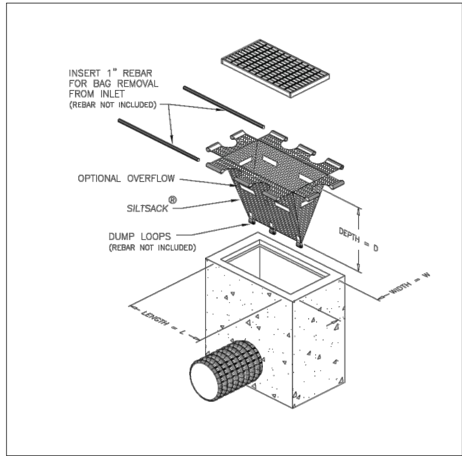
FILTER BAG DETAL NTS
