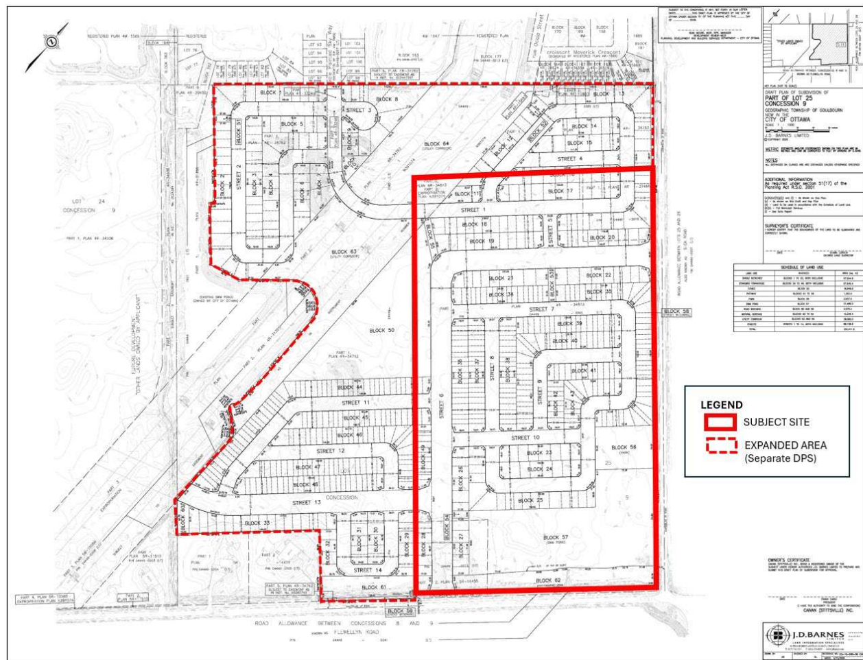
Figure 9 – Draft Plan
