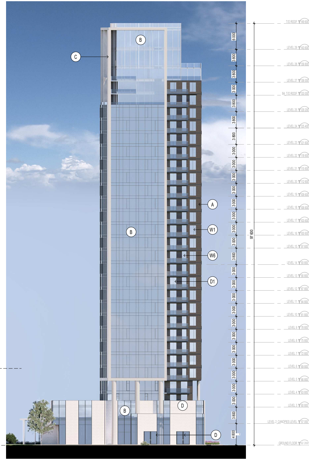
SOUTH ELEVATION_B1
