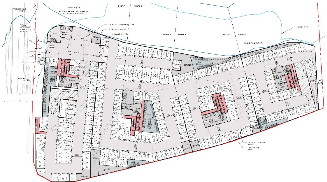
Figure 16: P2 Parking Plan (NEUF Architects)
