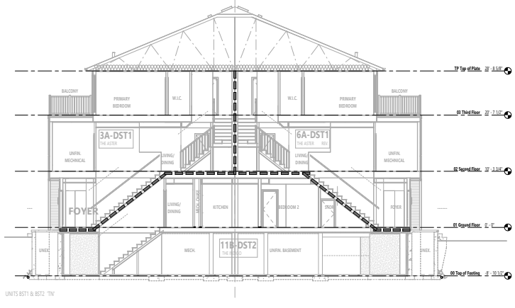
BUILDING SECTION B-B
